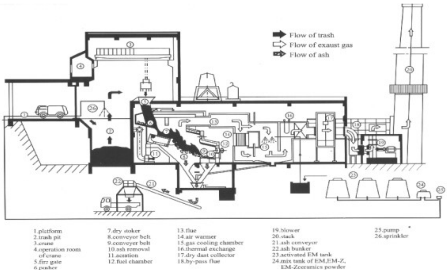
Fig 3. Flow Diagram of the Gushikawa Municipal Incinerator
