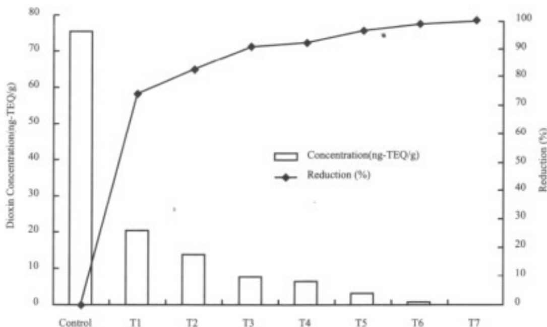
Fig 4. Reduction of Dioxins (PCDD/PCDF) Emission by EM Materials at the Gushikawa Municipal Waste Incinerator
