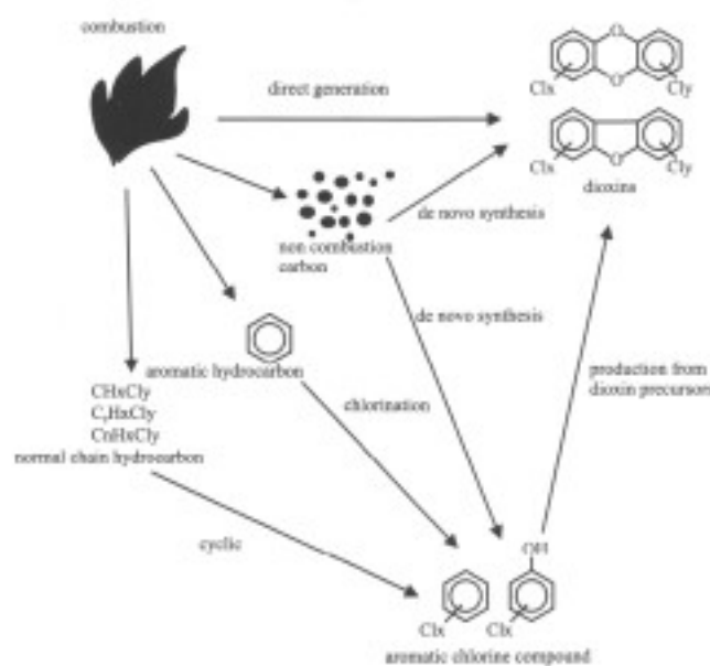
Fig 2. Main Sources of Dioxin Production through Combustion in Trash Incinerators
